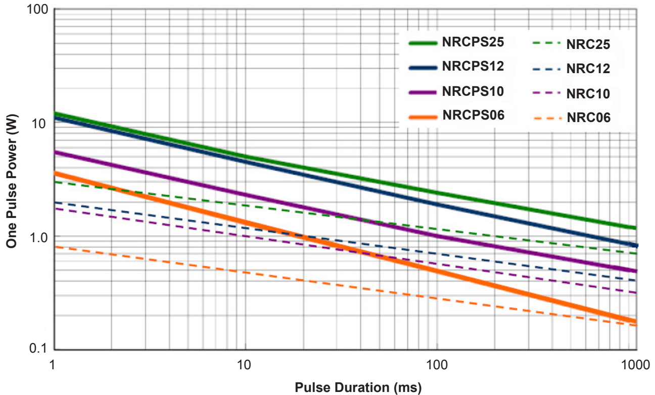
Single Pulse Power Characteristics NRCPS vs. NRC Series
